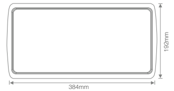
Recessed base
