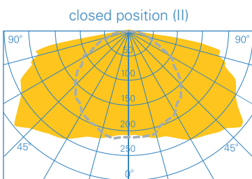
Closed position (II) suggested application for Escape Route, up to 9,5m in 4m height
