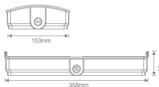
Weatherproof base
